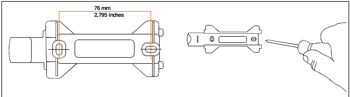
Figure 12- Wall-mounting adapter
